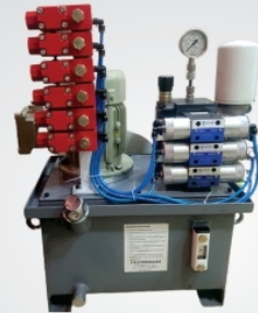
Flame Proof Hydraulic Power Pack Unit.
