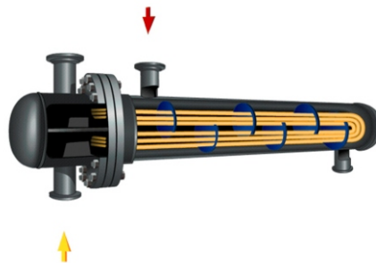
U-Tube-Heat-Exchanger
